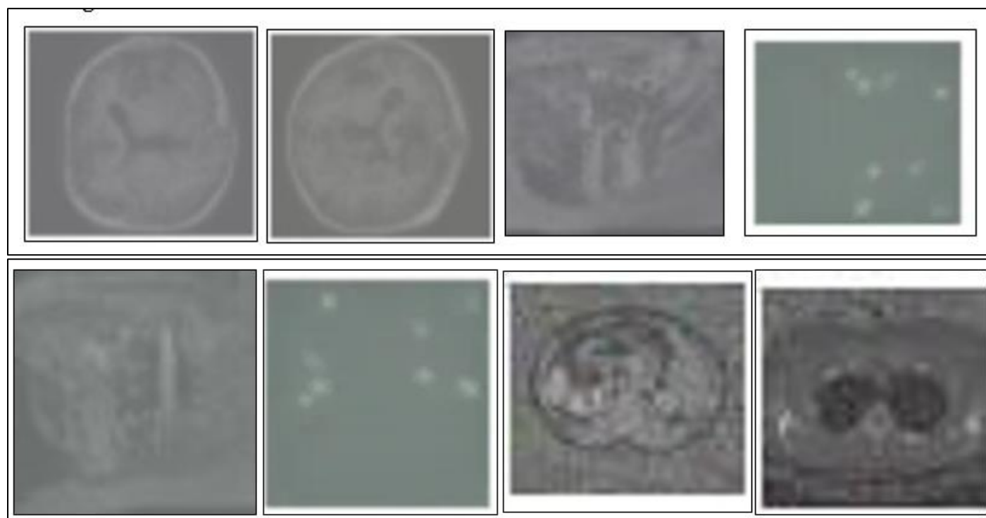
Fig 11: Generated Images
