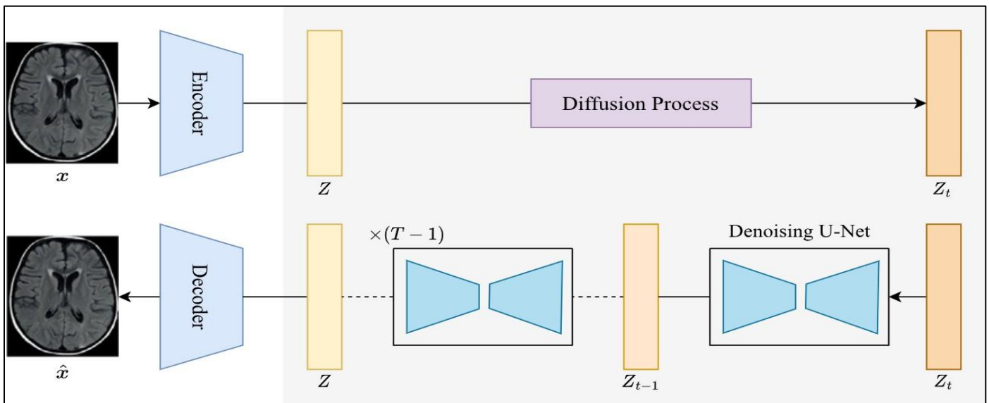
Fig 7: Architecture
